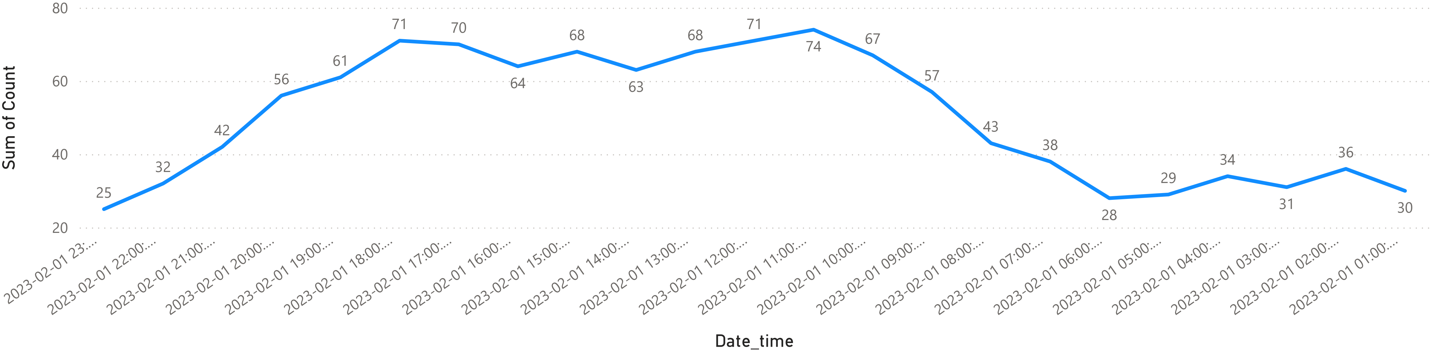
Incident Forecasting
